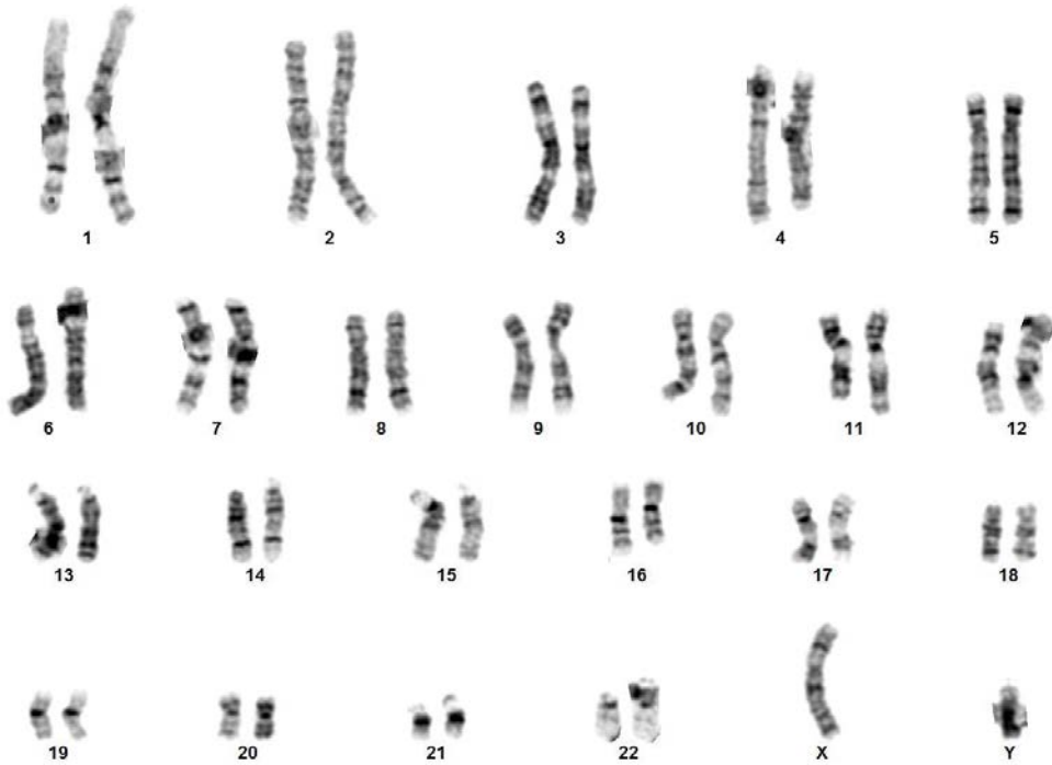
Figure 5. G-banding karyogram
